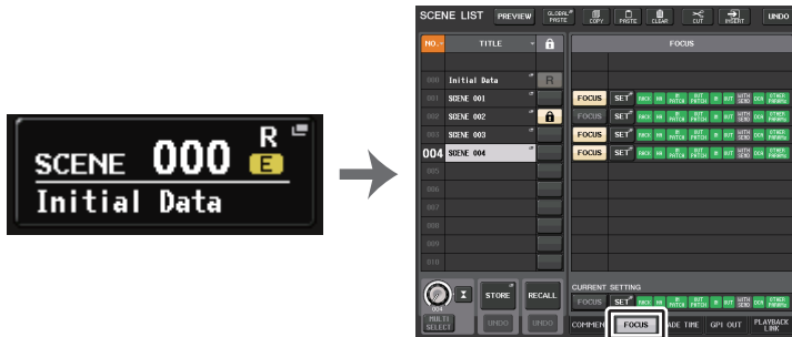
Поле SCENE
