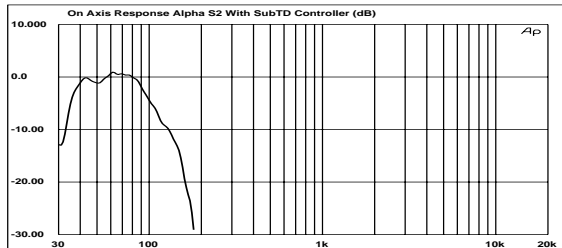
• Figure 1: Frequency Response with Sub TDcontroller (dB)
