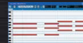
Piano Roll
